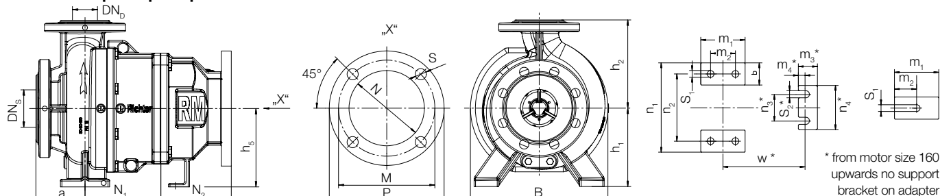
Pump dimensions in mm (inch)
