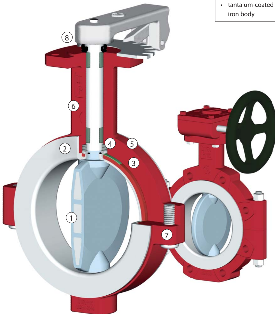
Wafer-style body NKS, NKS-C
