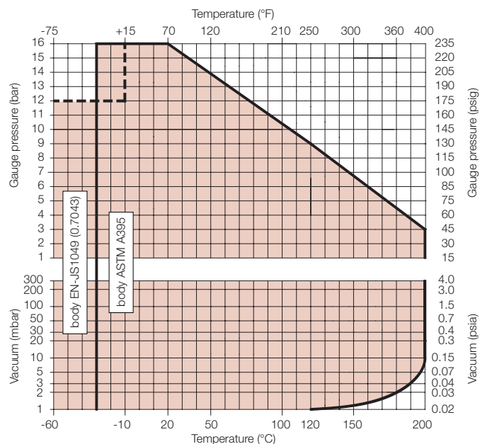
Pressure/temperature range
