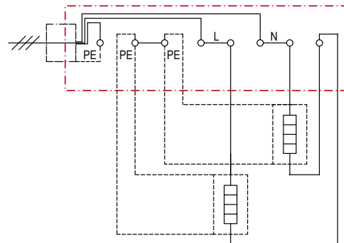
Connected in series with splice kit
