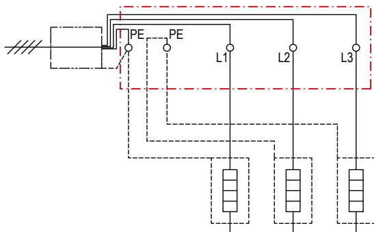
3 phases connected
