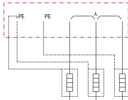
Star configuration
